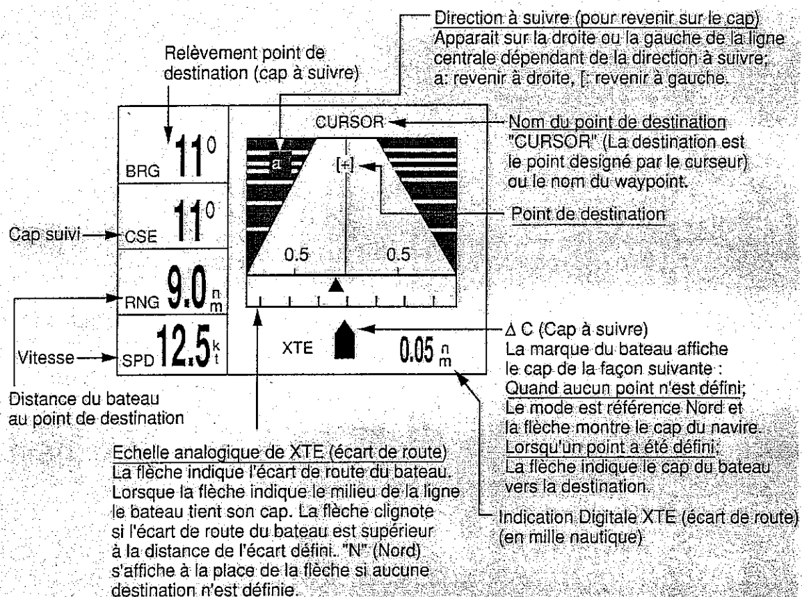
Figure 1-5 Affichage piste 3D
