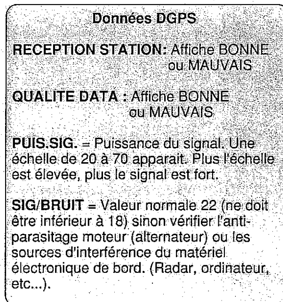
Figure 7-6 menu PARAMETRE DGPS
